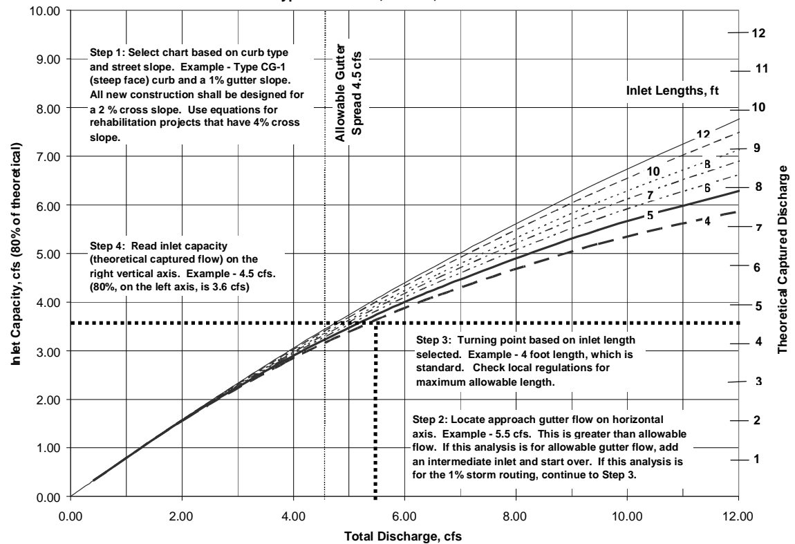
Figure 5604-3 (DESIGN EXAMPLE) Type CG-1 Curb, S_x=2\% , S_o=1.0\%
