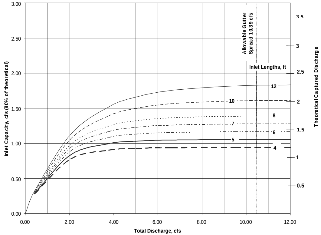
Figure 5604-19 Type CG-2 Curb, Sx=2%, So=12.0 %
