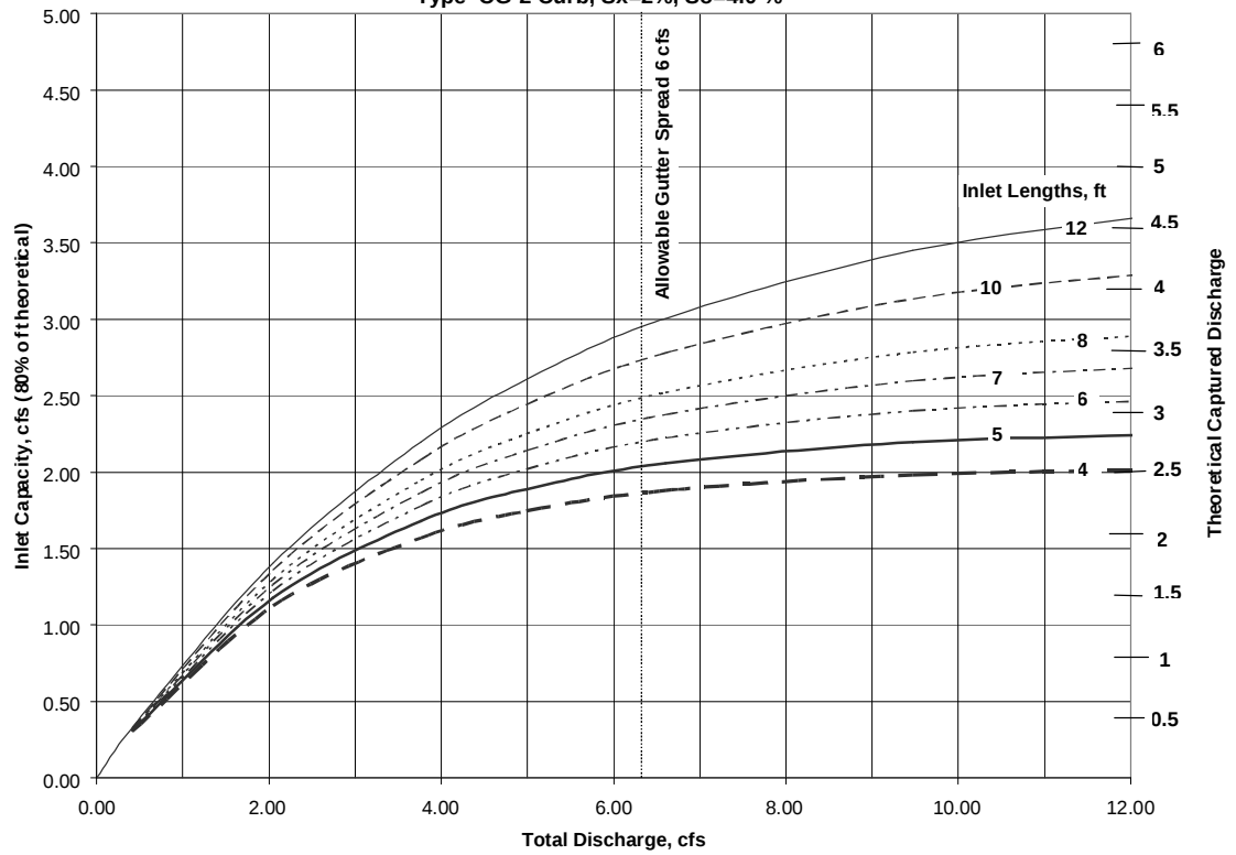
Figure 5604-15 Type CG-2 Curb, Sx=2%, So=4.0 %
