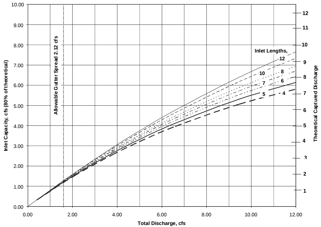
Figure 5604-11 Type CG-2 Curb, S_x=2\% , S_o=0.5\%
