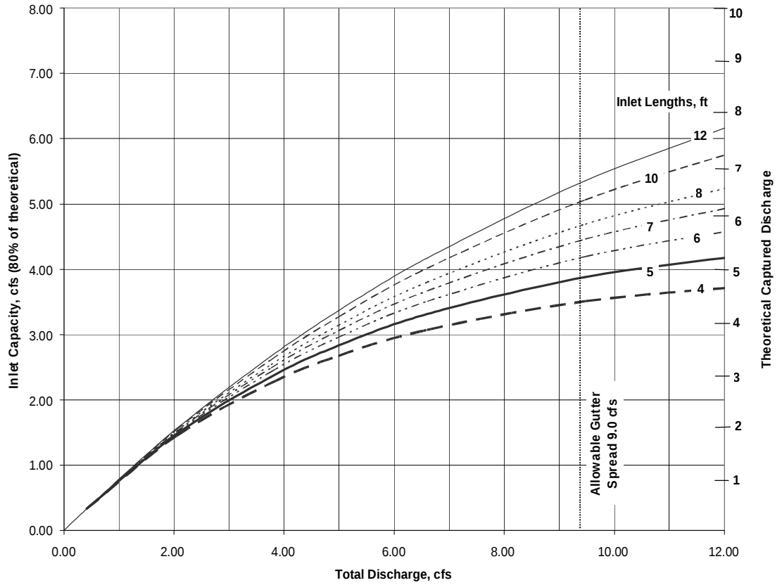
Figure 5604-6 Type CG-1 Curb, Sx=2%, So=4.0 %
