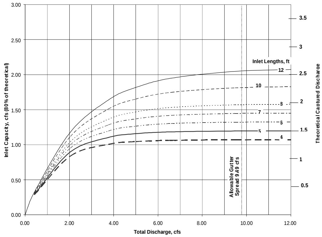
Figure 5604-18 Type CG-2 Curb, Sx=2%, So=10.0 %
