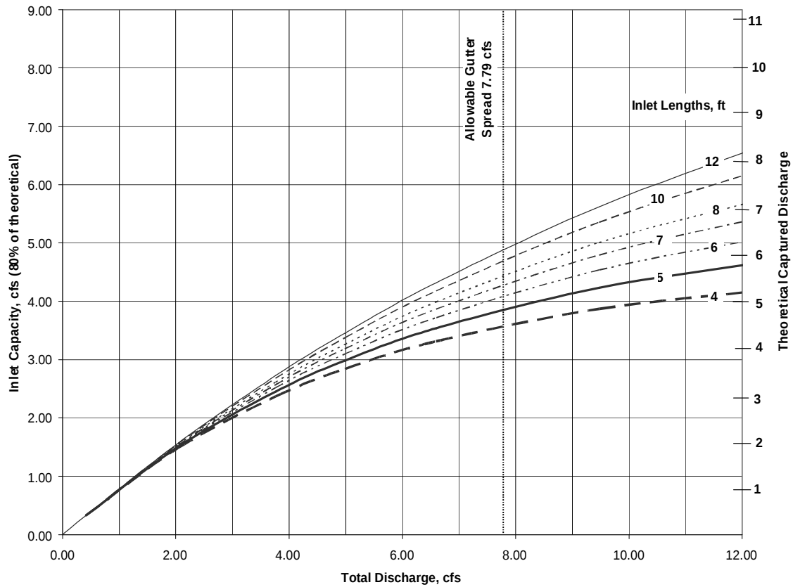
Figure 5604-5 Type CG-1 Curb, Sx=2%, So=3.0 %
