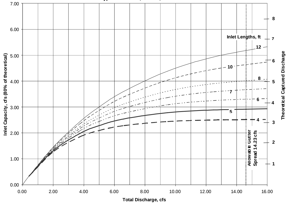
Figure 5604-9 Type CG-1 Curb, Sx=2%, So=10.0 %
