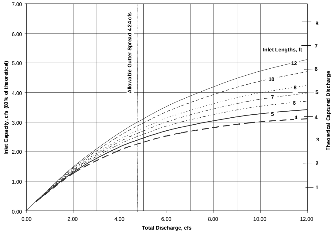
Figure 5604-13 Type CG-2 Curb, Sx=2%, So=2.0 %
