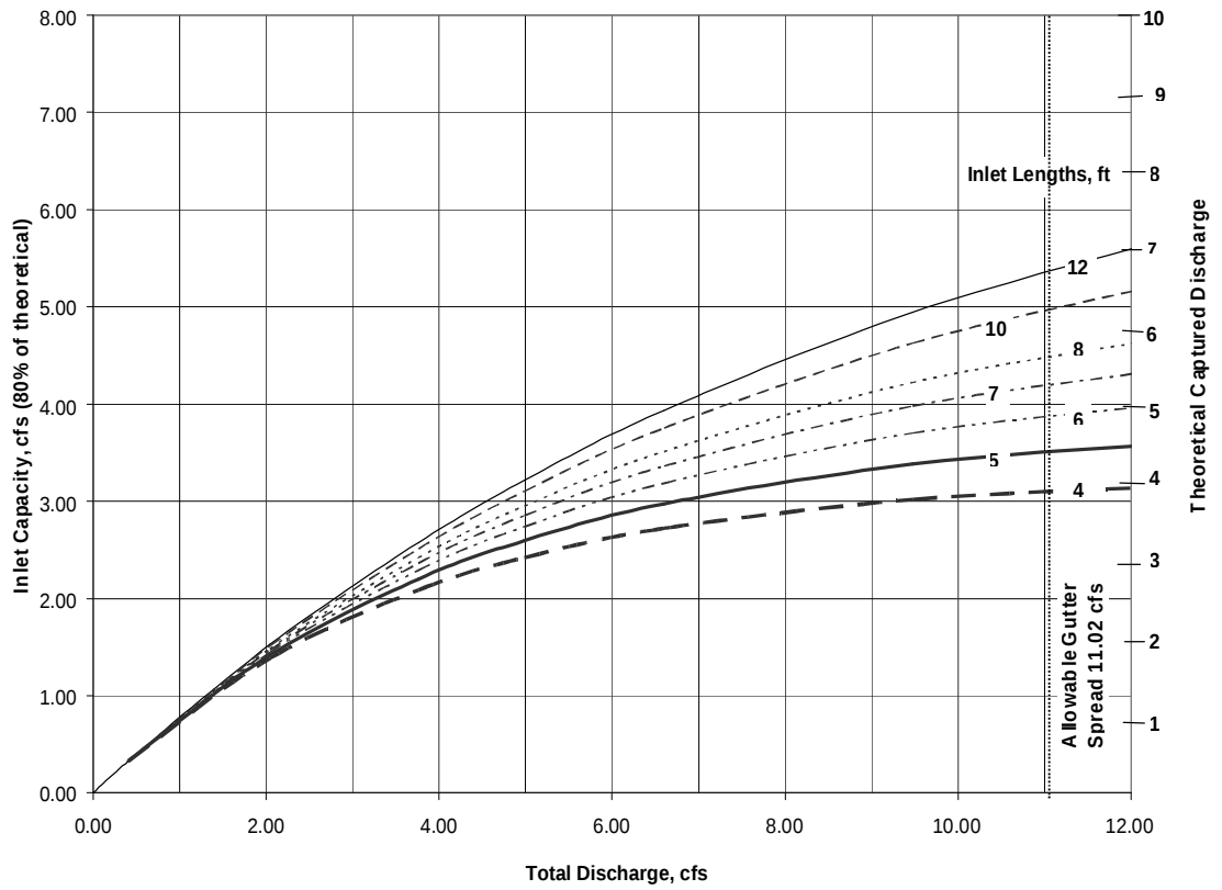
Figure 5604-7 Type CG-1 Curb, Sx=2%, So=6.0 %
