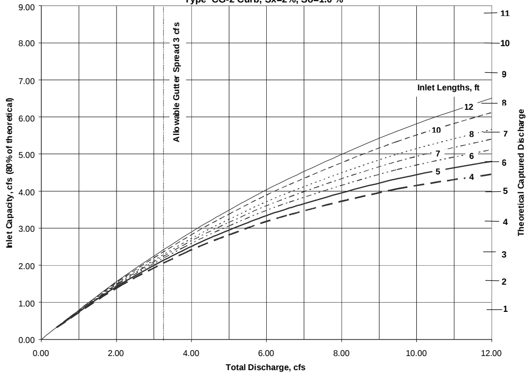
Figure 5604-12 Type CG-2 Curb, Sx=2%, So=1.0 %
