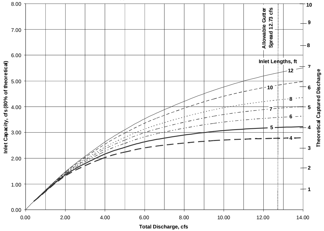
Figure 5604-8 Type CG-1 Curb, Sx=2%, So=8.0 %
