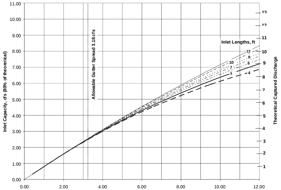
Figure 5604-3 (DESIGN EXAMPLE) Type CG-1 Curb, S_x=2\% , S_o=1.0\%
