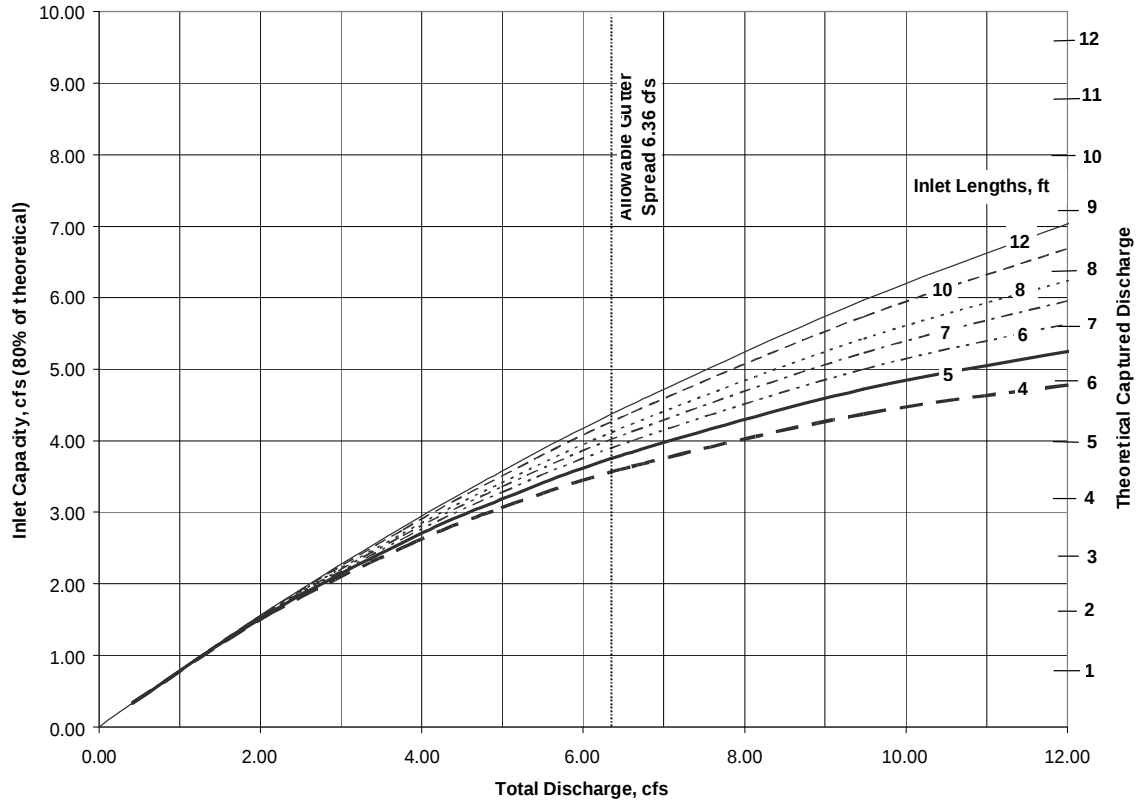
Figure 5604-4 Type CG-1 Curb, Sx=2%, So=2.0 %
