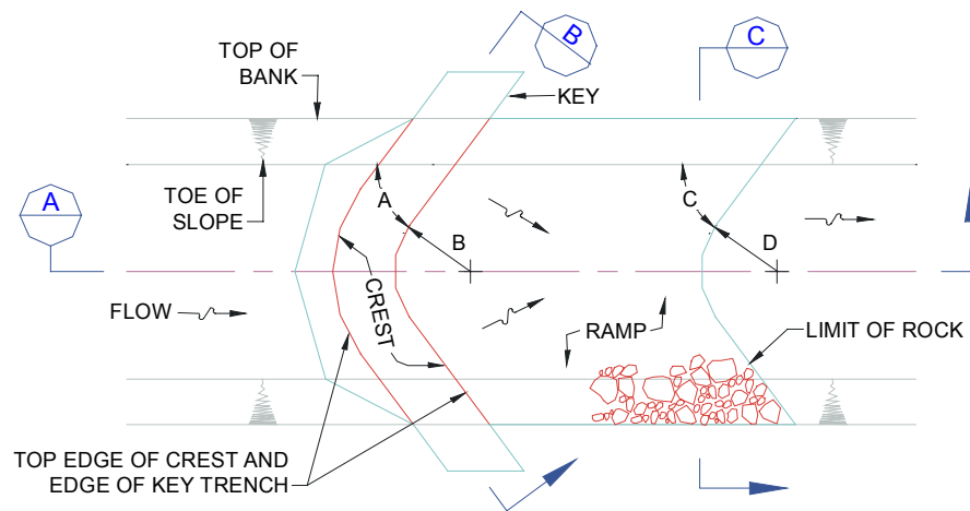
Figure 5605-3: Grade Control Structure
