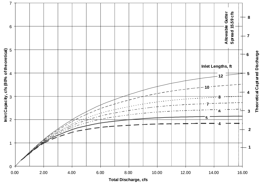
Figure 5604-10 Type CG-1 Curb, S_x=2\% , S_o=12.0\%
