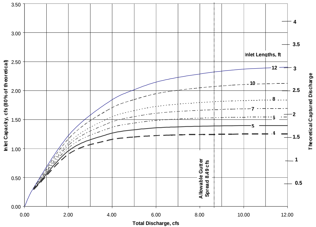
Figure 5604-17 Type CG-2 Curb, Sx=2%, So=8.0 %
