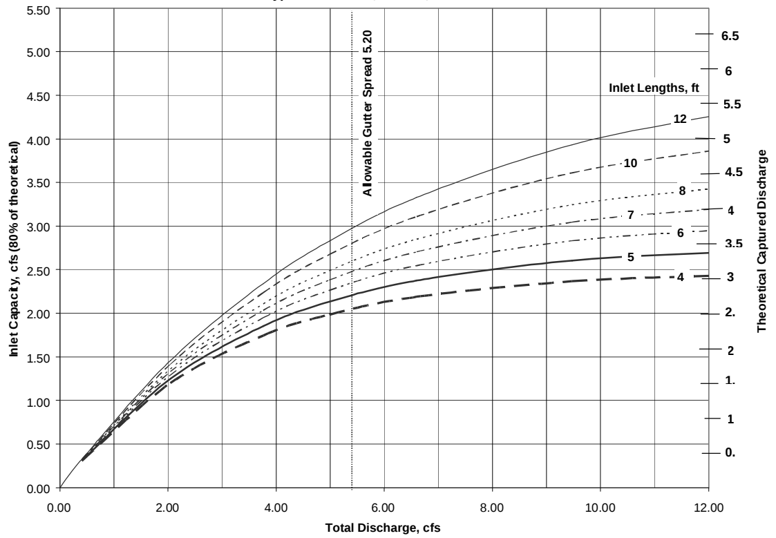
Figure 5604-14 Type CG-2 Curb, Sx=2%, So=3.0 %
