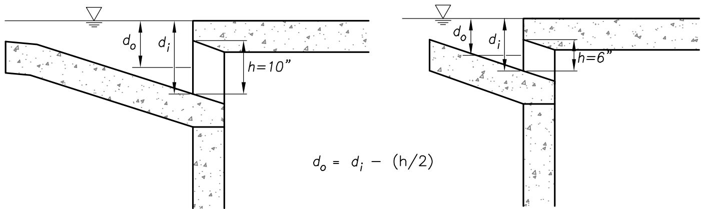
TYPE 1 CURB INLET
