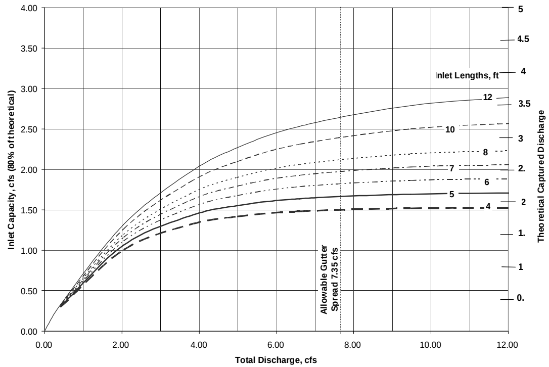
Figure 5604-17 Type CG-2 Curb, Sx=2%, So=8.0 %
